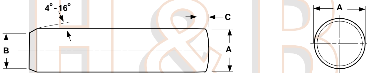
DOWEL PINS, STANDARD SERIES
