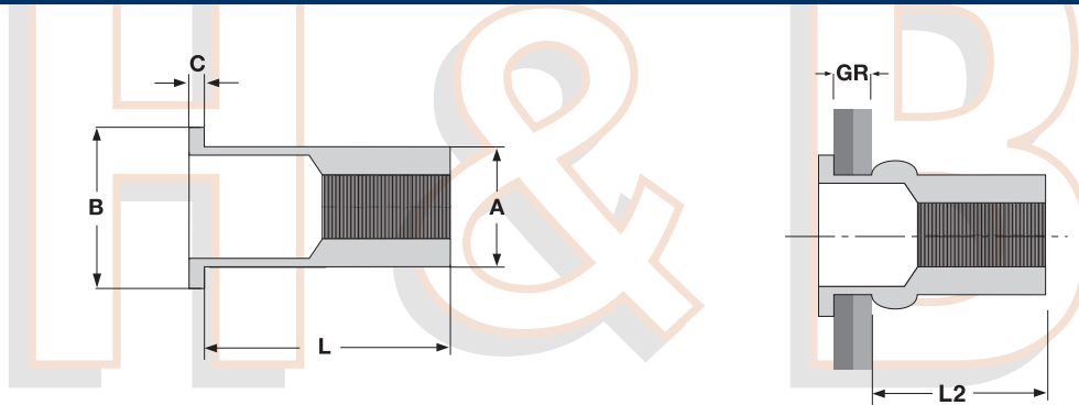
FLAT HEAD, NON-RIBBED BLIND THREADED INSERT
