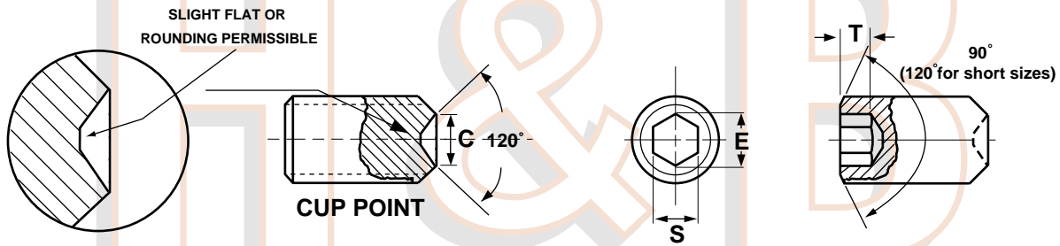
METRIC - SOCKET SET SCREWS, CUP POINT
